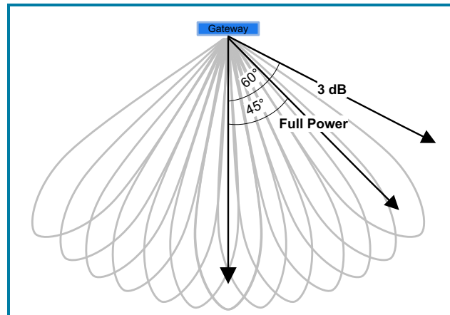
Figure 3: Full transmit power coverage area of 90° and 3dB beamwidth at 120°
