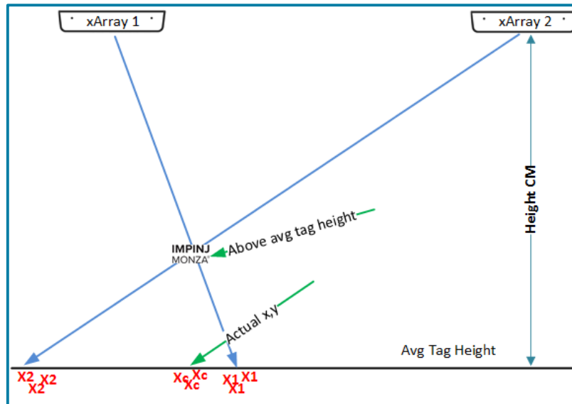
Figure 38: Weighted Tag Average Height Measurement, Near and Far xArray Scenario
