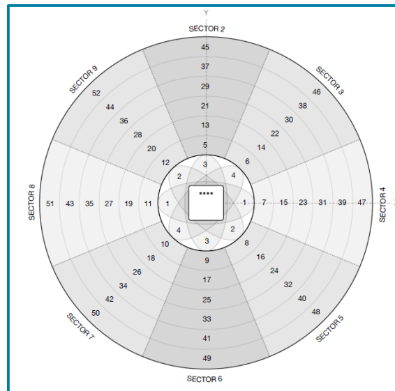
Figure 82: xArray 52 beam, 9 sectors
