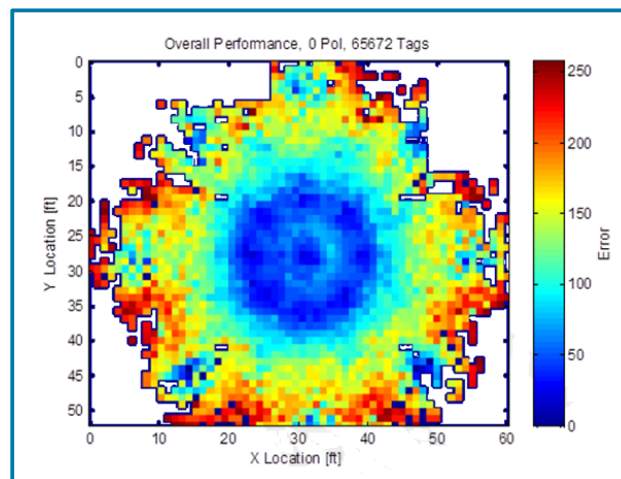
Figure 35: Location Accuracy Heatmap
