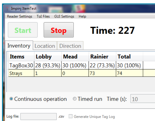
Figure 64: Tag Read percents by xArray
