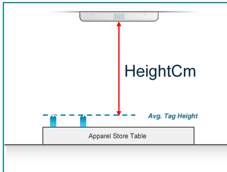
Figure 39: xArray HeightCM Measurement vs Avg. Tag Height
