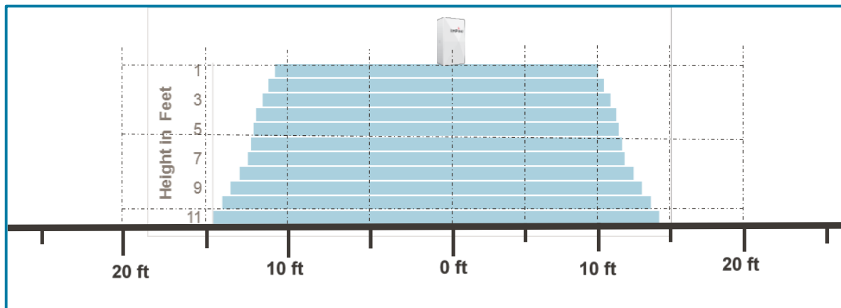
Figure 8: xSpan Minor Axis Coverage Diagram
