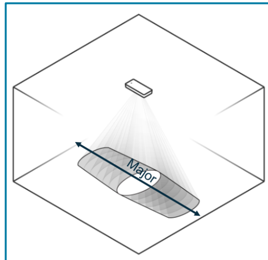
Figure 5: xSpan Coverage with Major Axis
