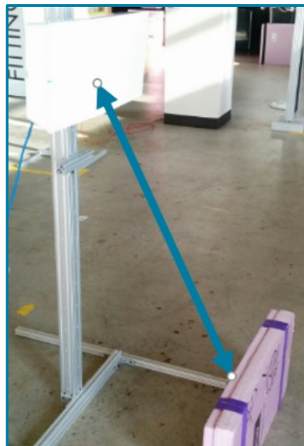
Figure 16: Horizontally Mounted xSpan Read Zone Test
