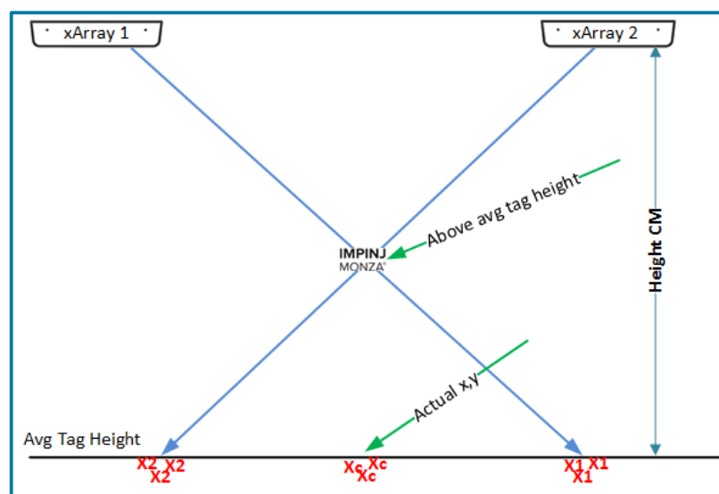
Figure 37: Weighted Tag Average Height Measurement, Two xArrays, Centered
